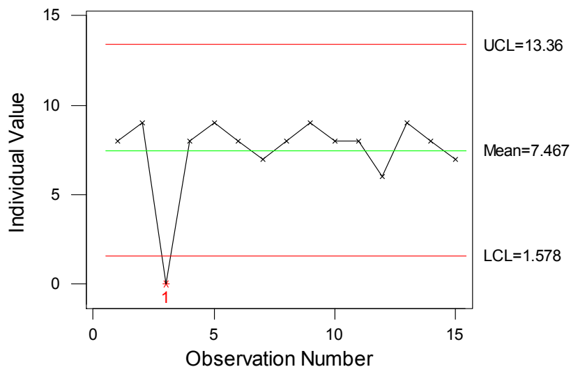
I Chart for Defects_
