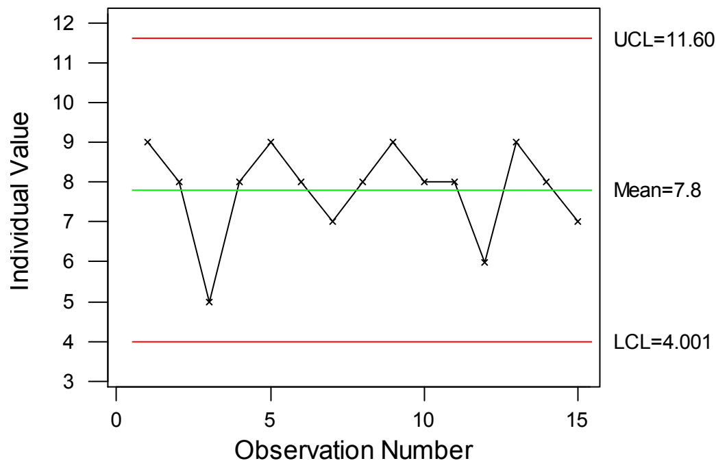
I Chart for Defects
