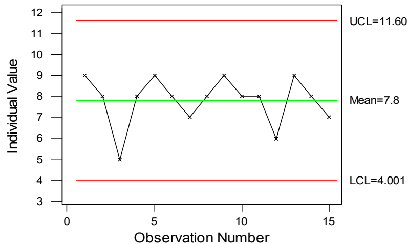
I Chart for Defects
