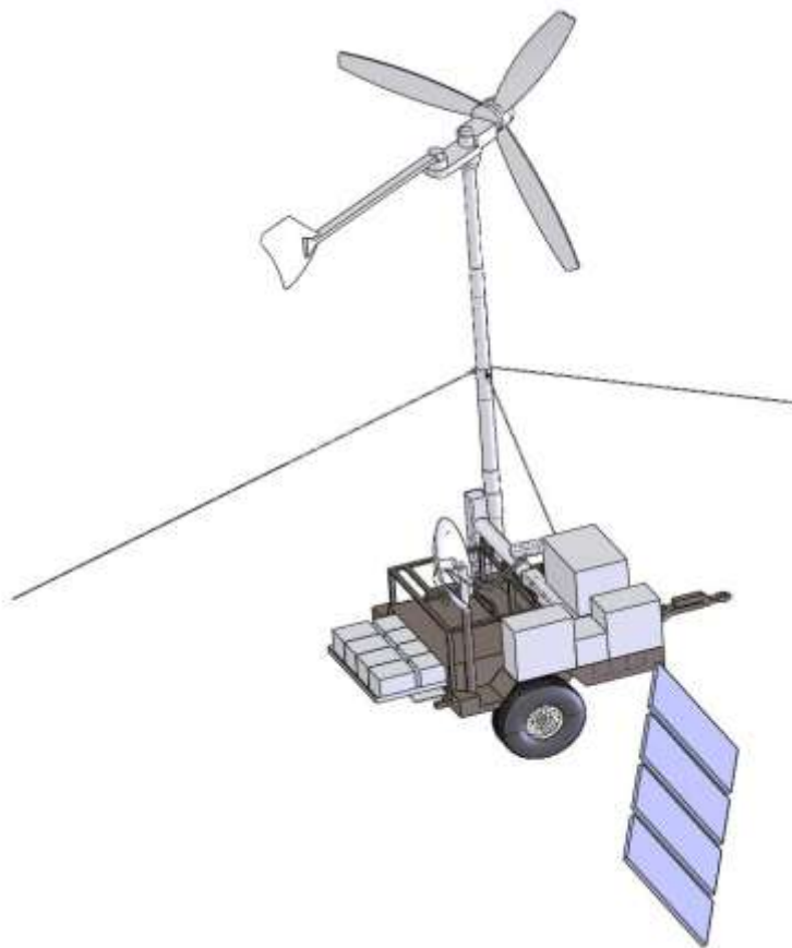
HERES - Deployed
