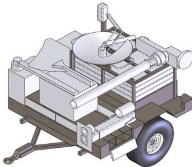
HERES - Stowed
