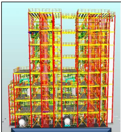
Holston AAP NAC/SAC Design
