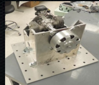
Hybrid Electric Power Unit
