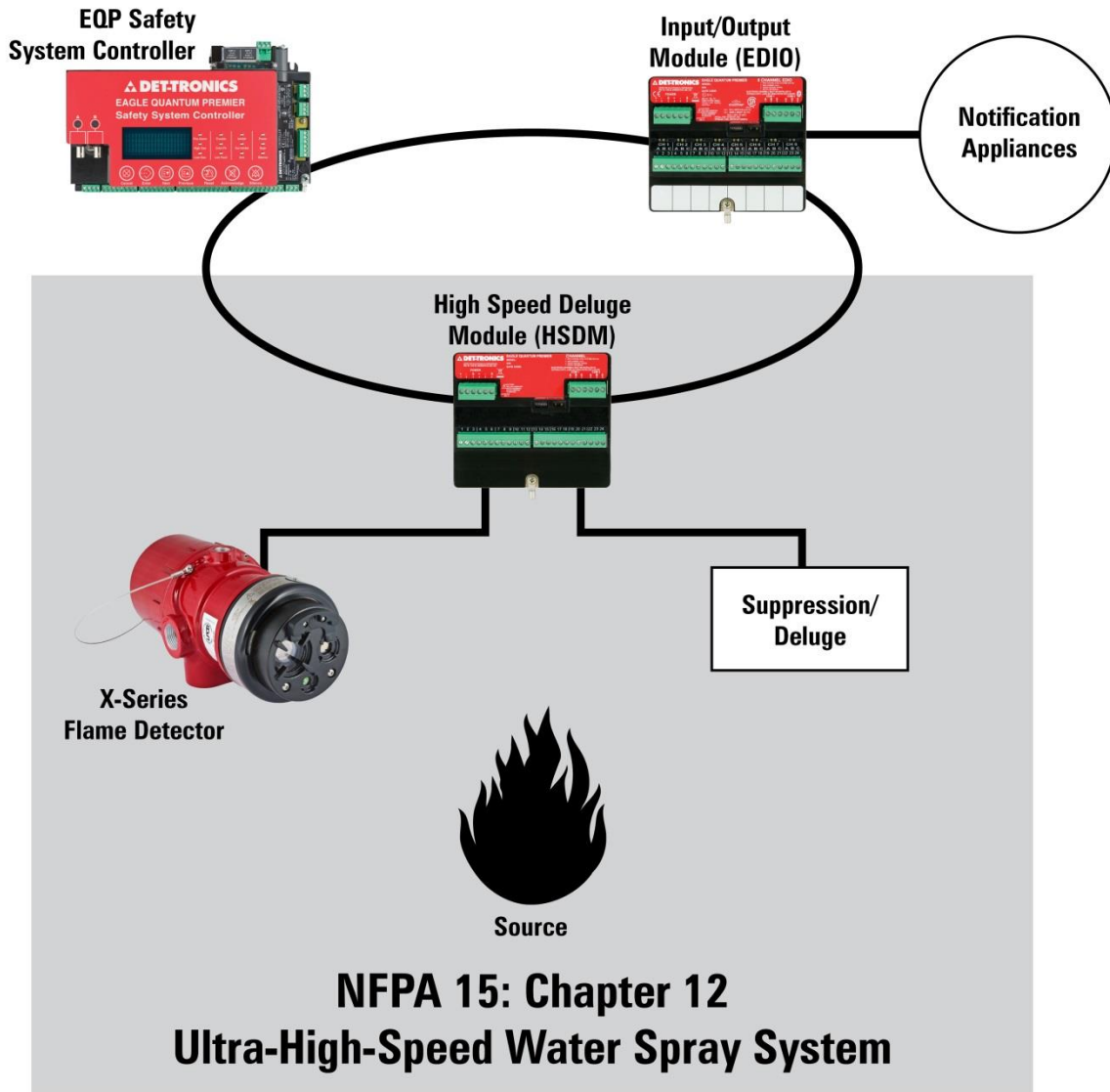
FIGURE 11: Visual depiction of an ultra-high-speed capable Det-Tronics system
