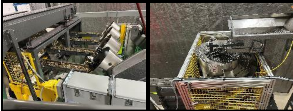
Cartridge Case Assembly & Component Feeders
